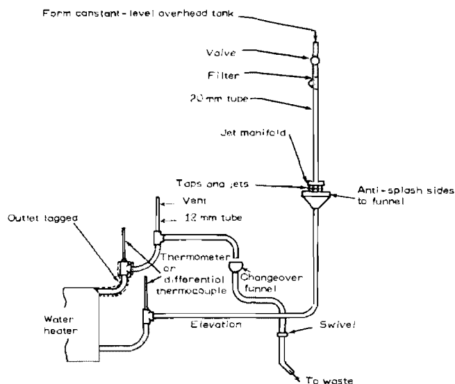
Fig. 2 - Typical Water Supply Connections for Tests
